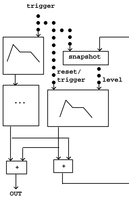
Figure 4.7: Block diagram for the switch-and-ramp technique.
